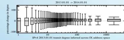
Figure 2. Figure 2 shows that for IPv4 ASes with degree less than 6, the median value of observed degree changes is 0, indicating that approximately equal numbers of those small ASes had their degree increased or decreased. ASes with degrees larger than 6 tended to increase their degree (medians in these bins are above 0). Yet in all degree
